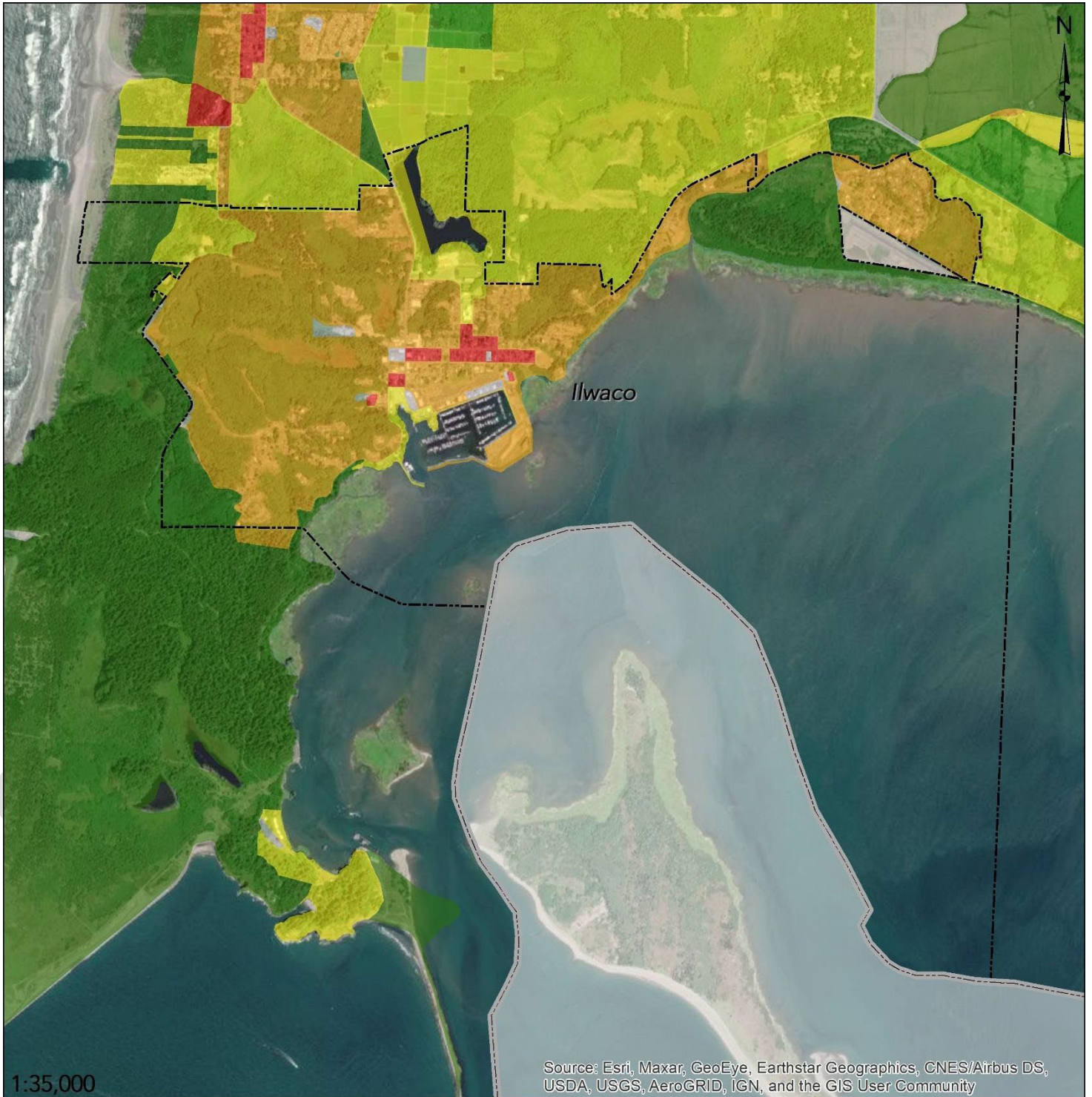
Map 3.24 – WUI, Ilwaco
