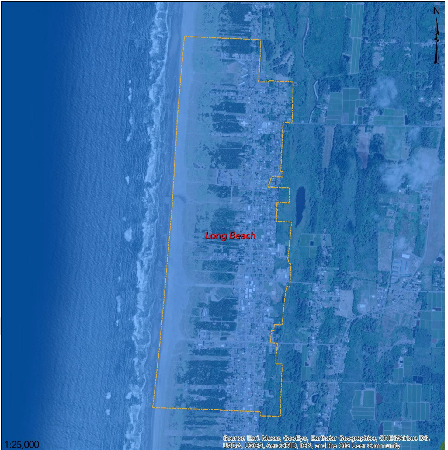
Map 3.17 – Cascadia Subduction Tsunami ~A.D. 1700 w/ Uplift, Long Beach
