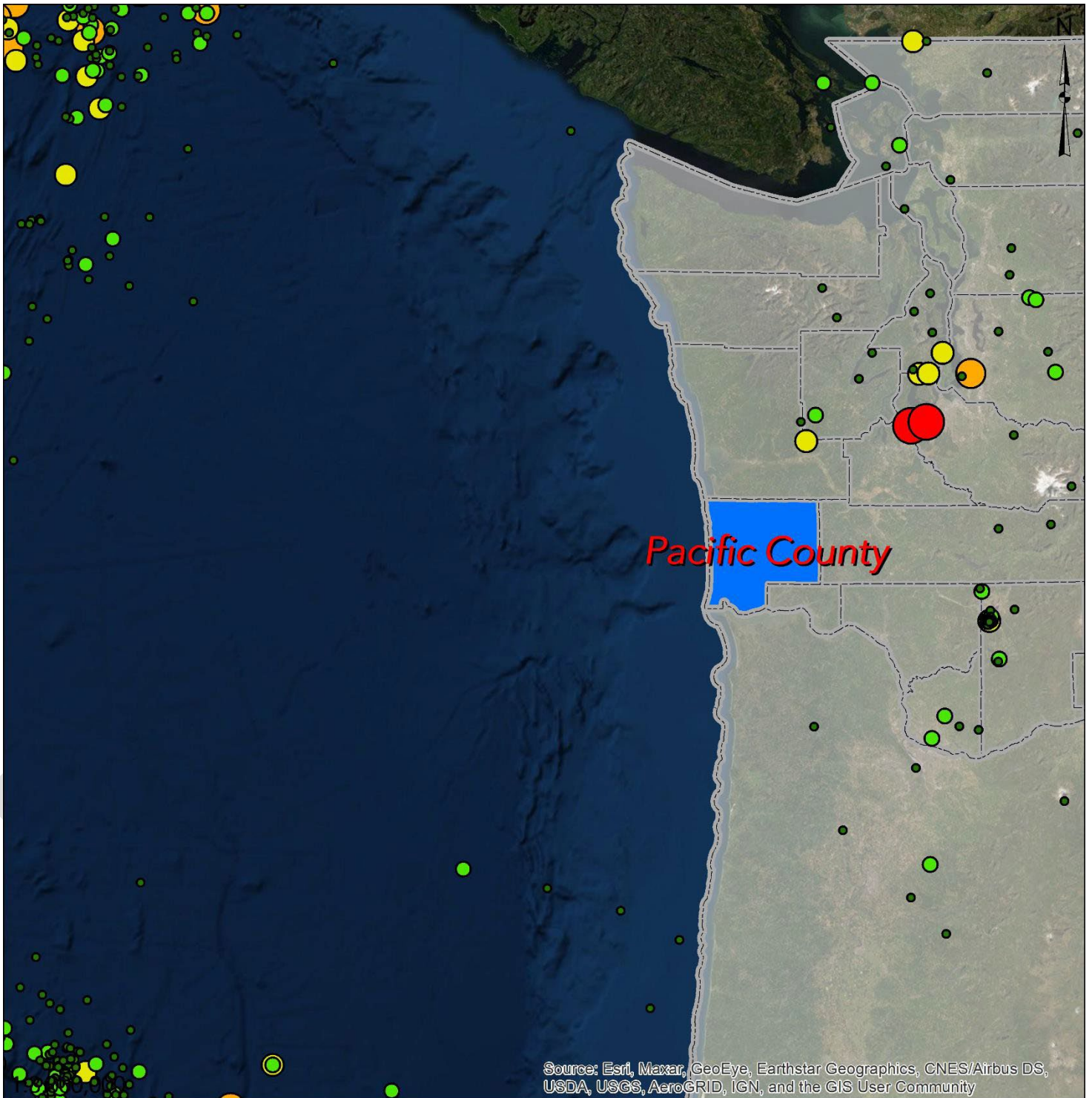
Map 3.3 – Historic Earthquakes, Pacific County
