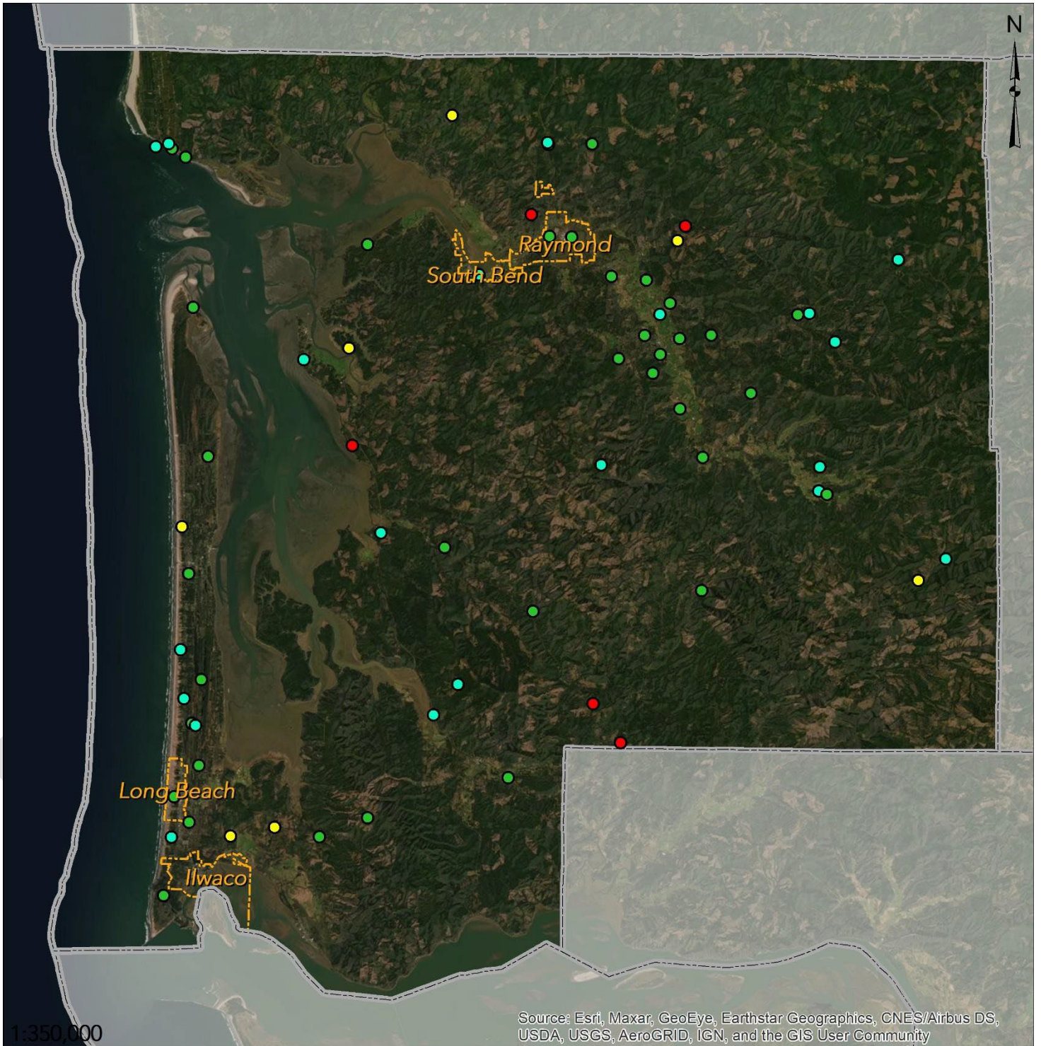
Map 3.28 – Historical Wildfires
