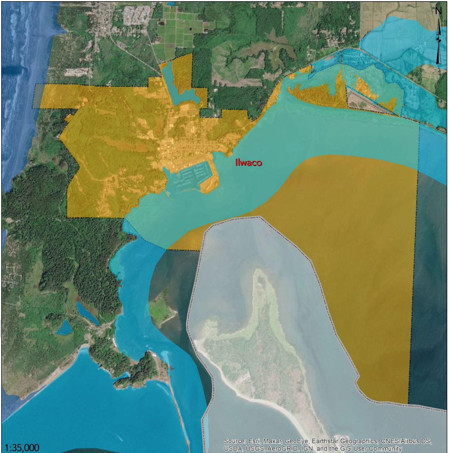
Map 3.7 – Floodplains, Ilwaco
