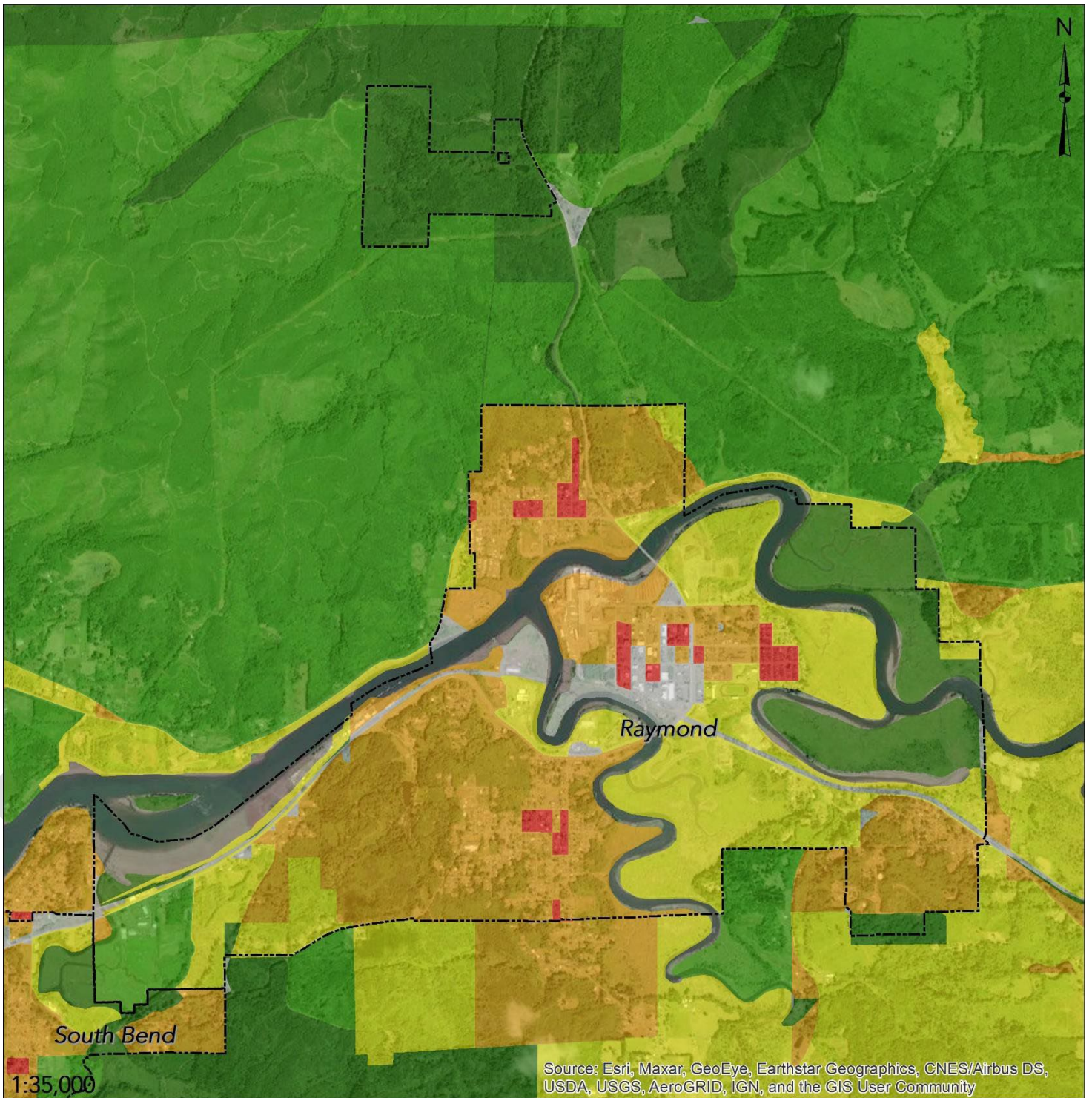
Map 3.26 – WUI, Raymond
