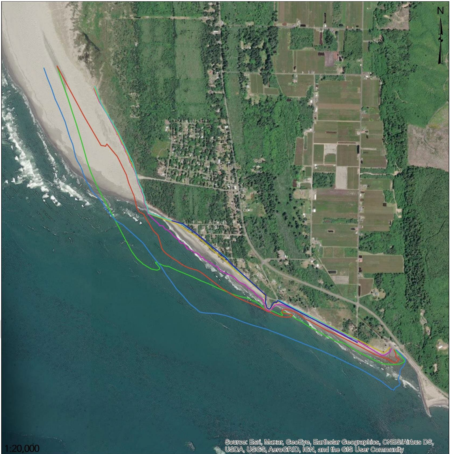
Map 3.1 – Coastal Erosion – Washaway Beach/North Cove Area
